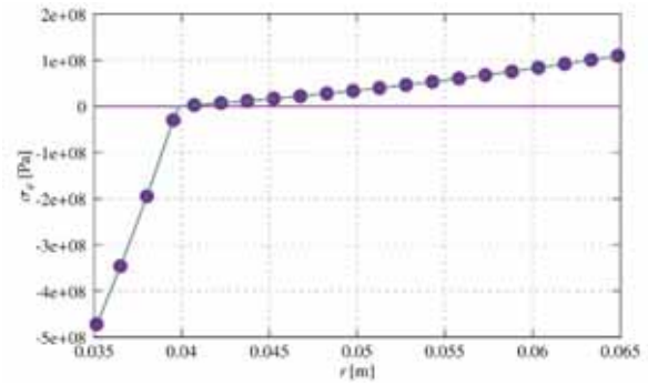
Figure 3 The graph of the circumferential normal stress.
