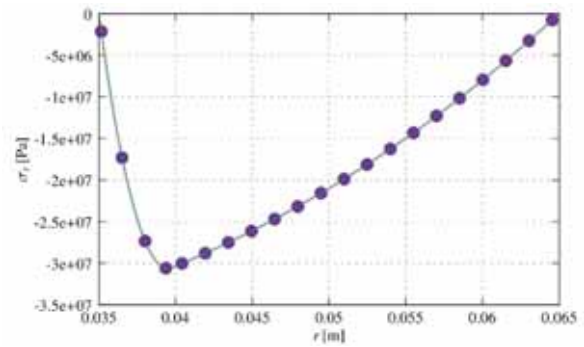
Figure 4 The plot of the radial normal stress.
