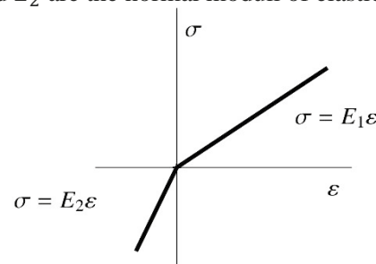
Figure 1 Stress-strain diagram.
