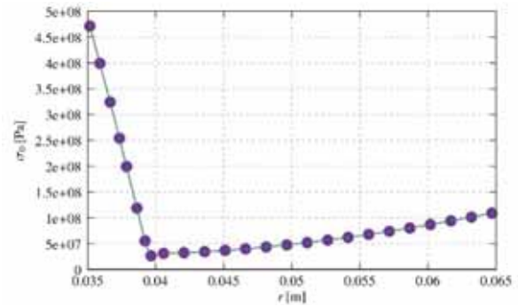
Figure 5 The plot of \sigma_0 = \sigma_0(r) .
